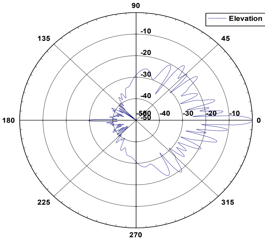
56 9004 Elevation Pattern
