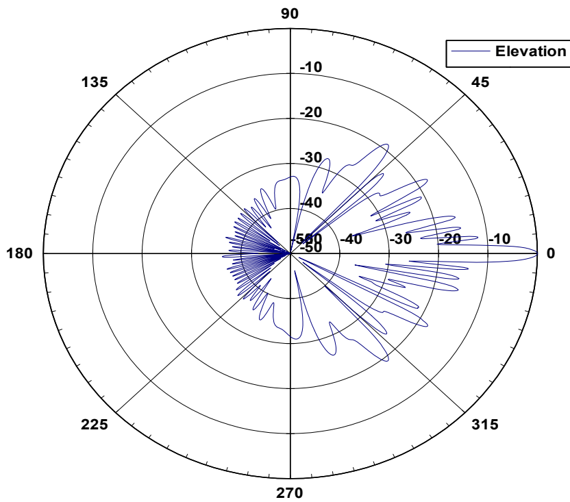
56 3004H Elevation Pattern
