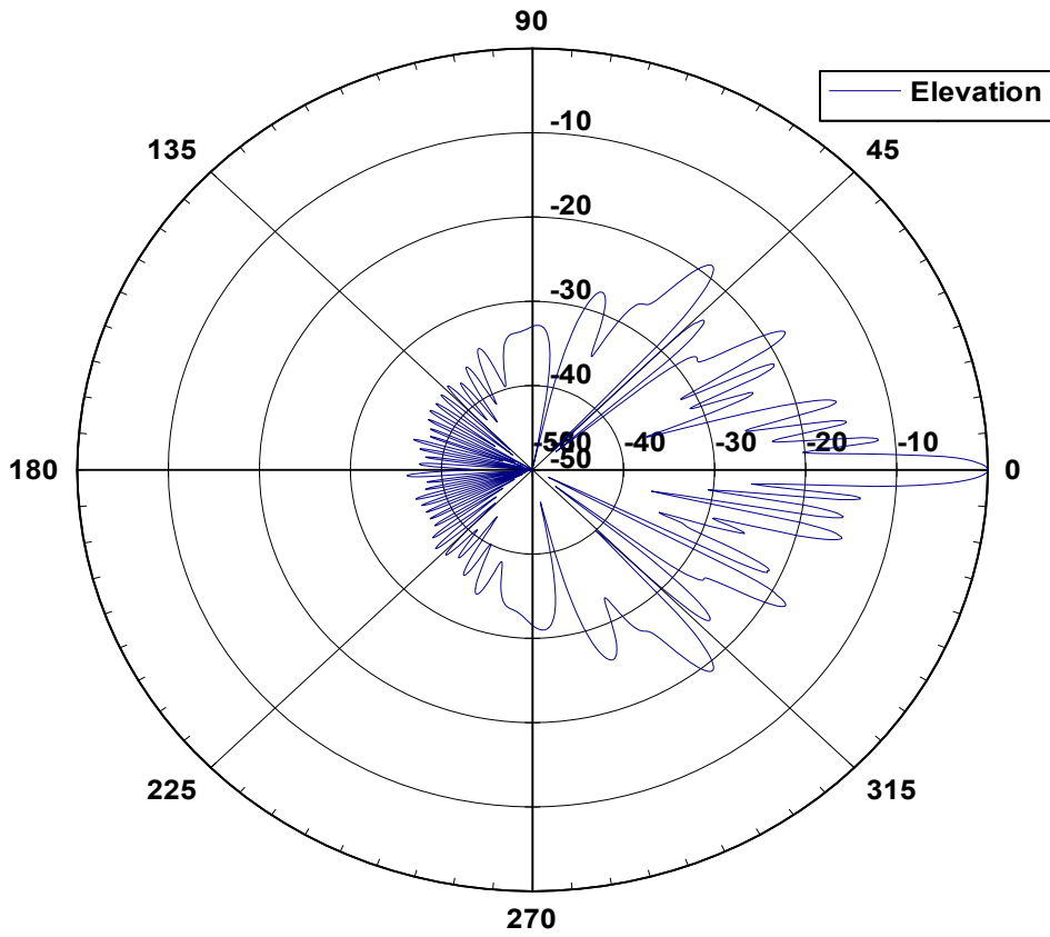
56 3004 Elevation Pattern
