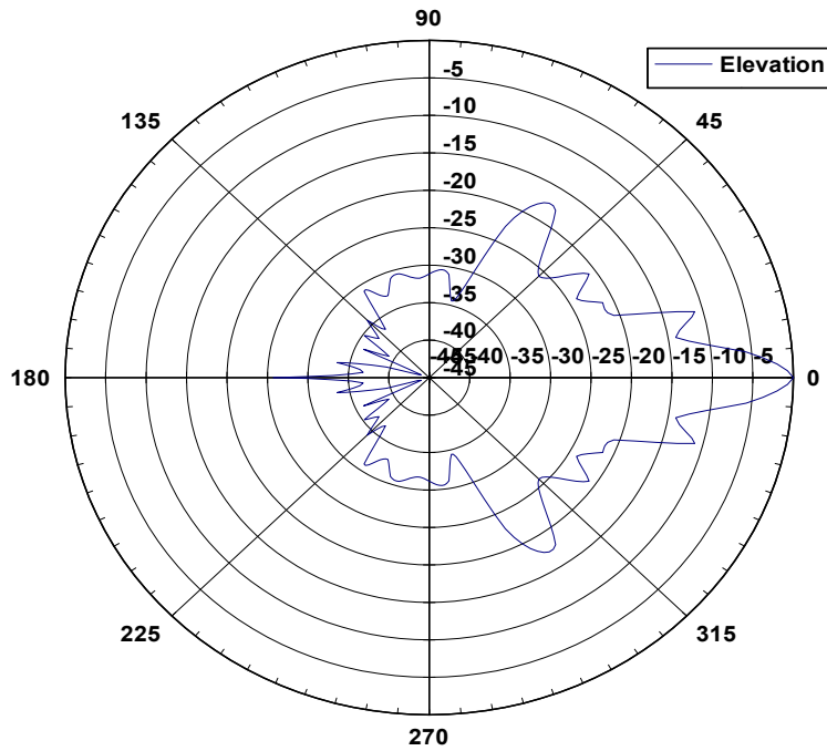
56 6010H Elevation Pattern
