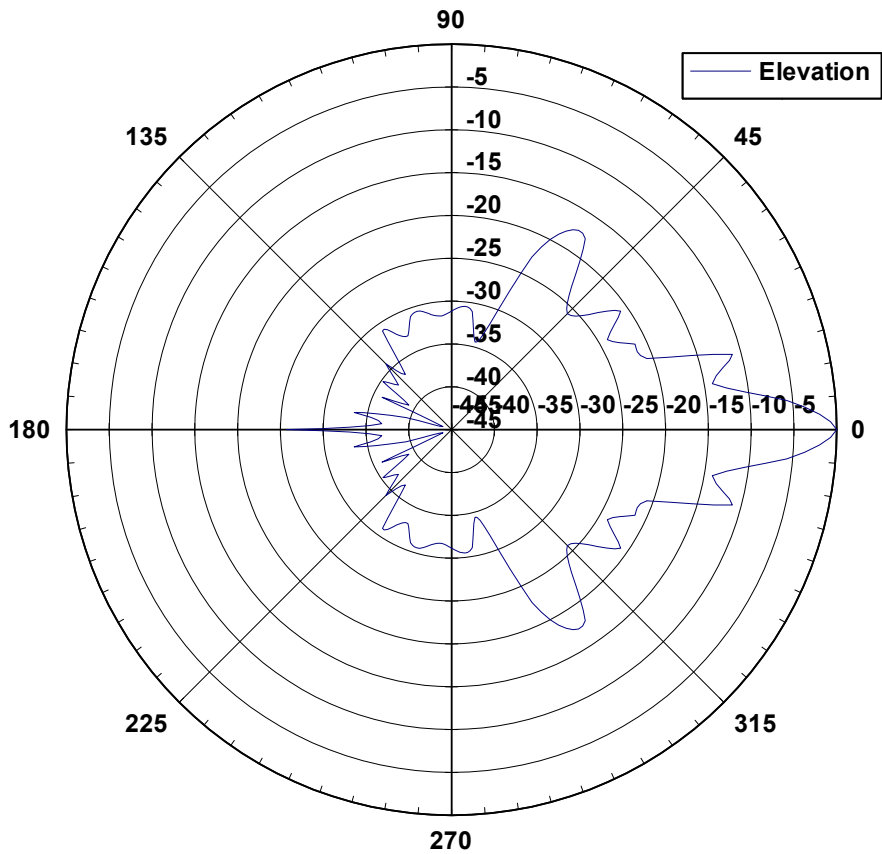
56 6010 Elevation Pattern
