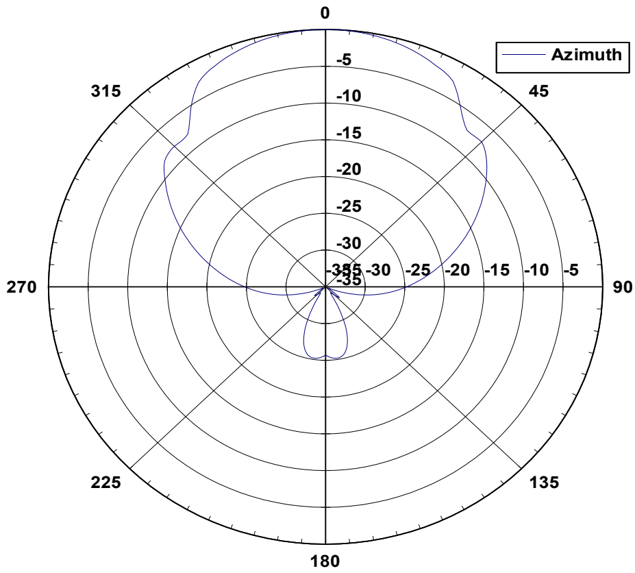
56 6010 Azimuth Pattern
