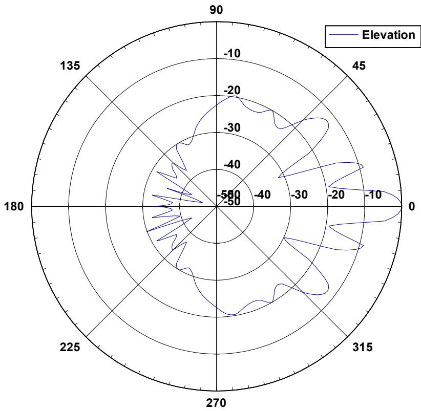
56 3010H Elevation Pattern
