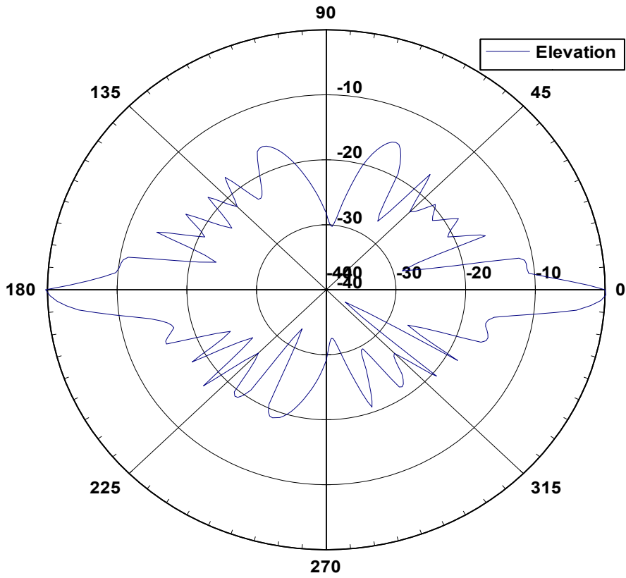
56 2360 Elevation Pattern
