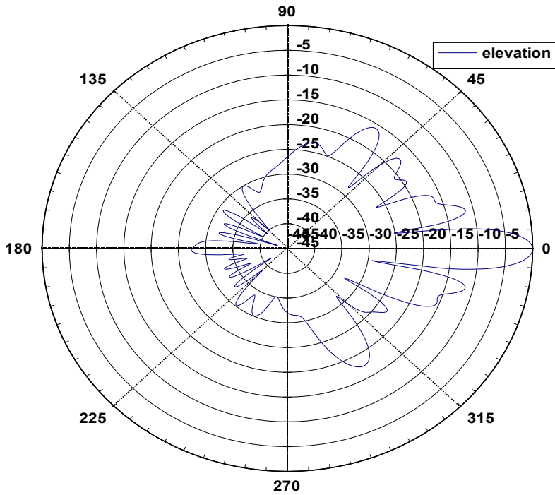
52 9010H Elevation Pattern
