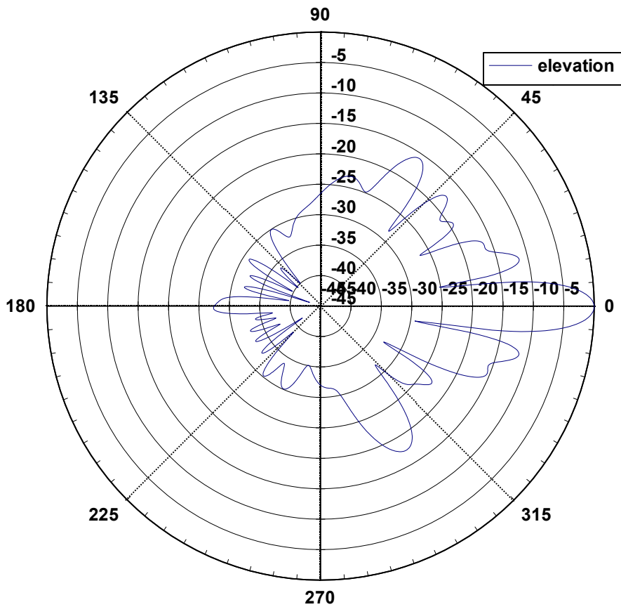
52 9010 Elevation Pattern
