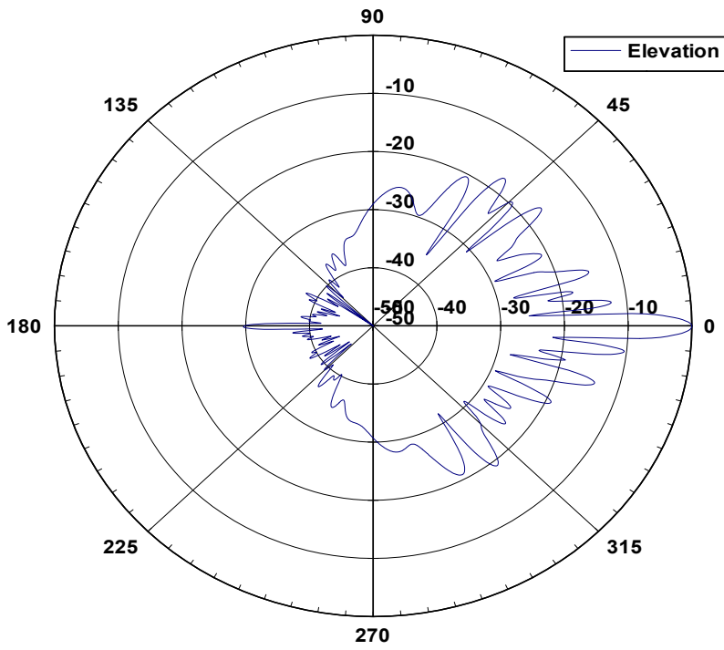
52 9004H Elevation Pattern
