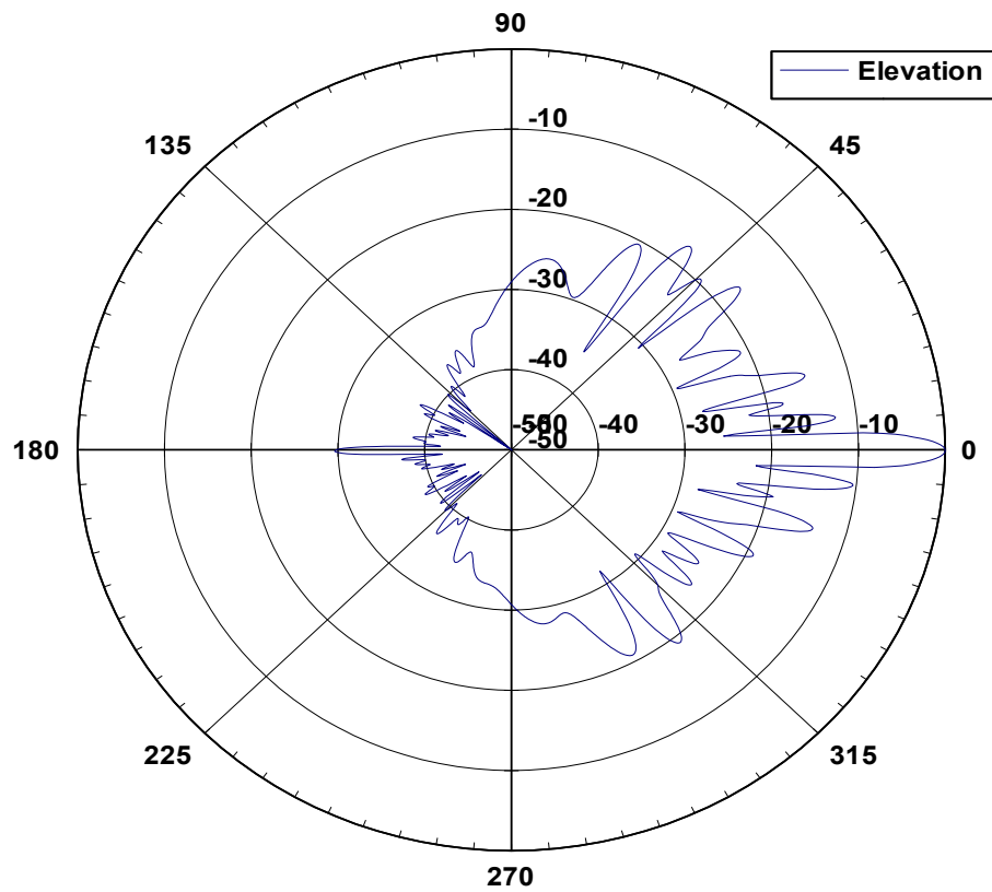
52 9004 Elevation Pattern
