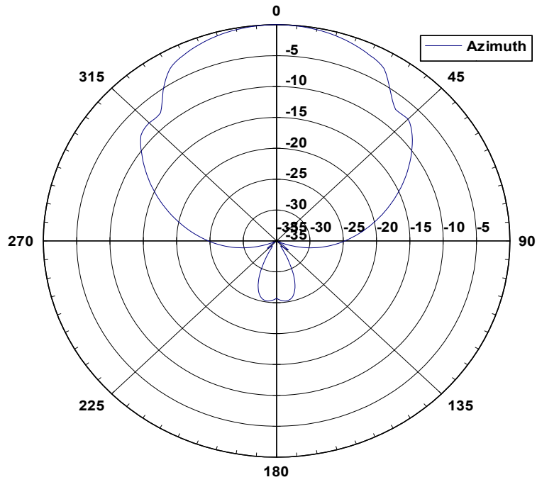
52 6010H Azimuth Pattern
