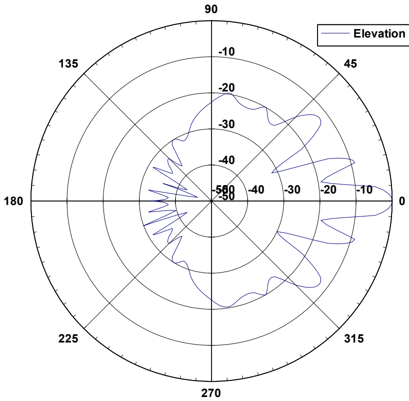
52 3008H Elevation Pattern
