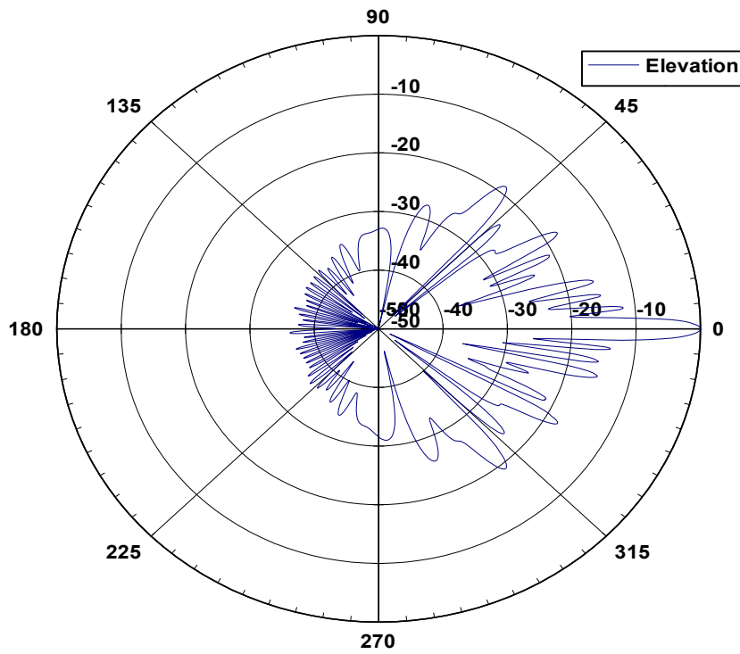
52 3004H Elevation Pattern
