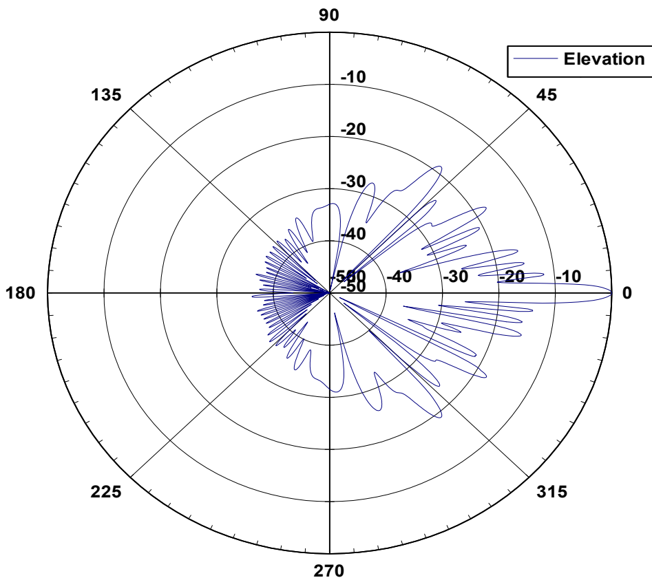
52 3004 Elevation Pattern
