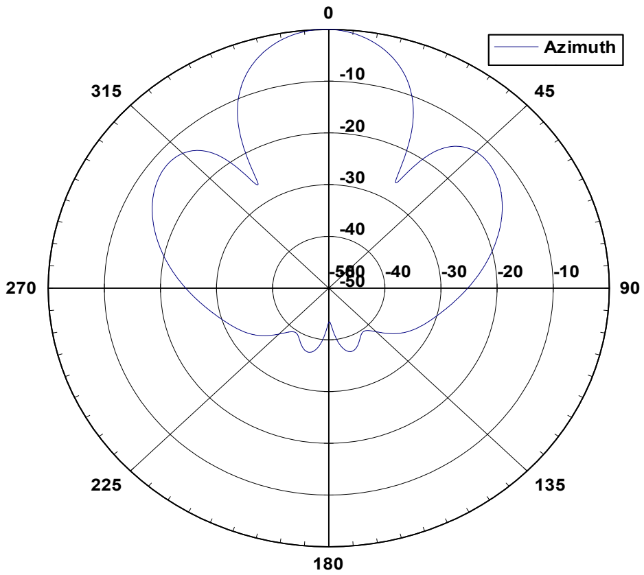
52 3004 Azimuth Pattern
