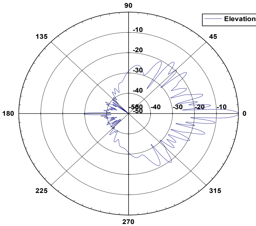
52 12005 Elevation Pattern
