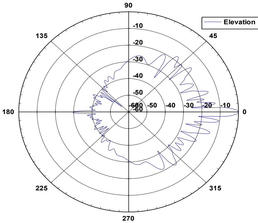
52 6004H Elevation Pattern
