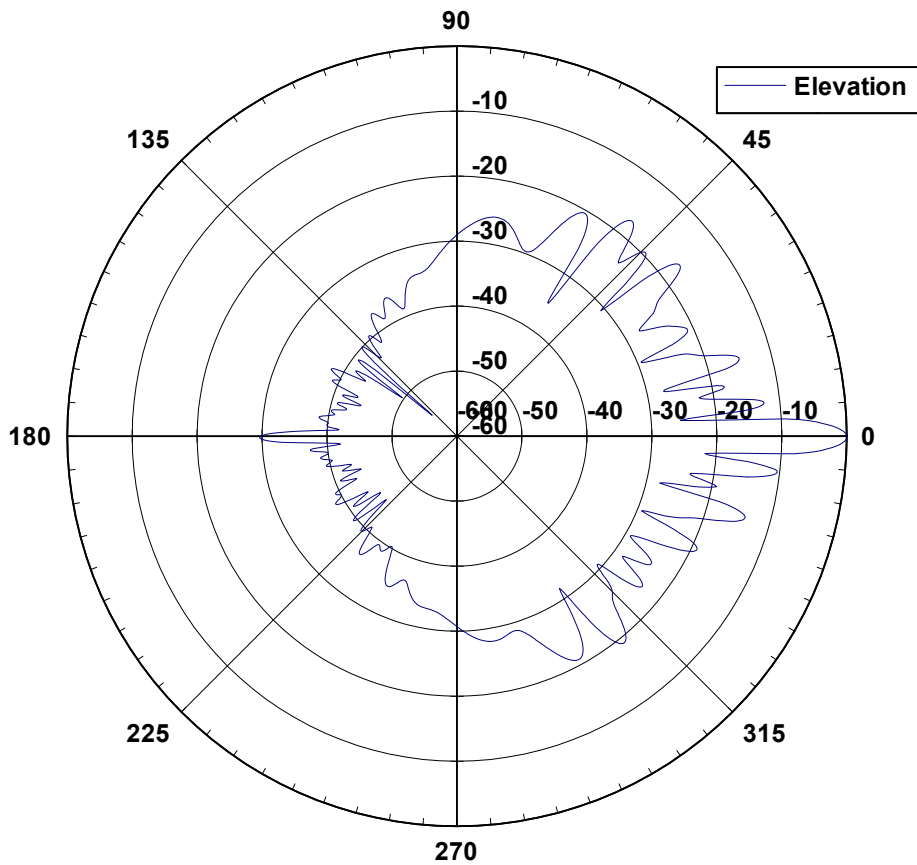
52 6004 Elevation Pattern
