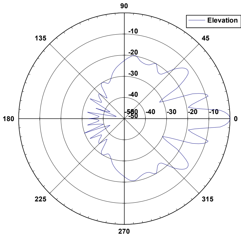
52 3008H Elevation Pattern
