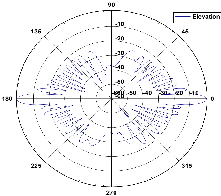
37 3360 Elevation Pattern
