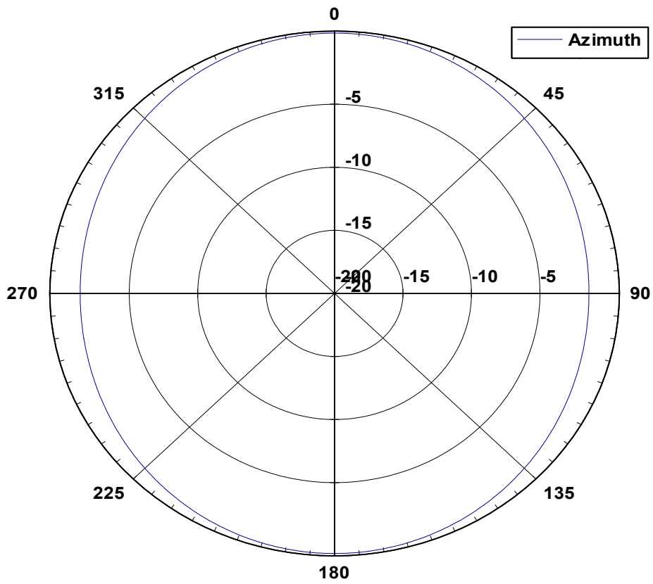
37 3360 Azimuth Pattern
