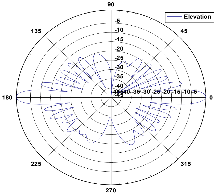
37 2360 Elevation Pattern
