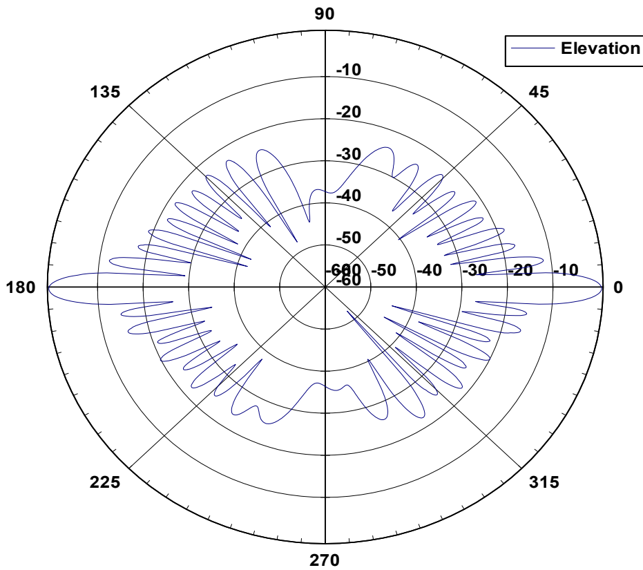
35 3360 Elevation Pattern
