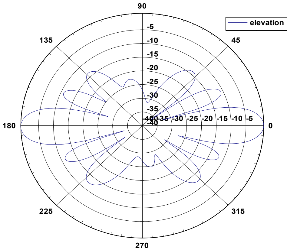
35 1360 Elevation Pattern
