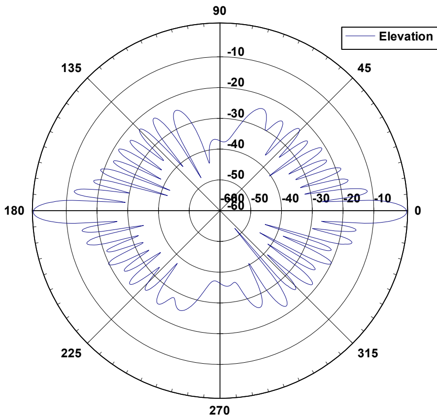
34 3360 Elevation Pattern
