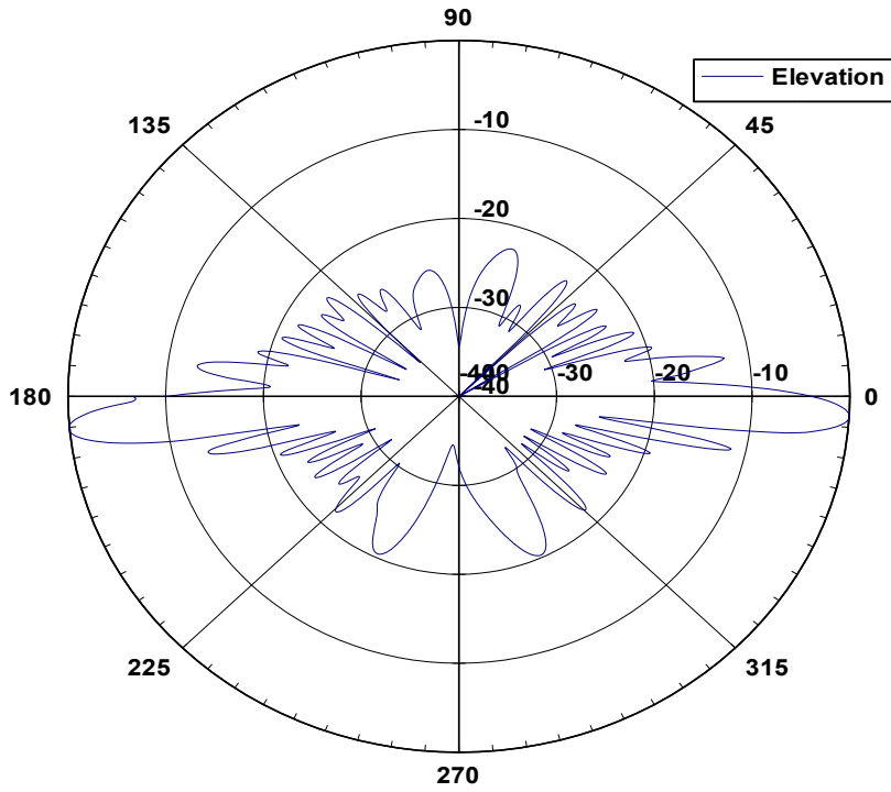
33 3360-2.5 Elevation Pattern
