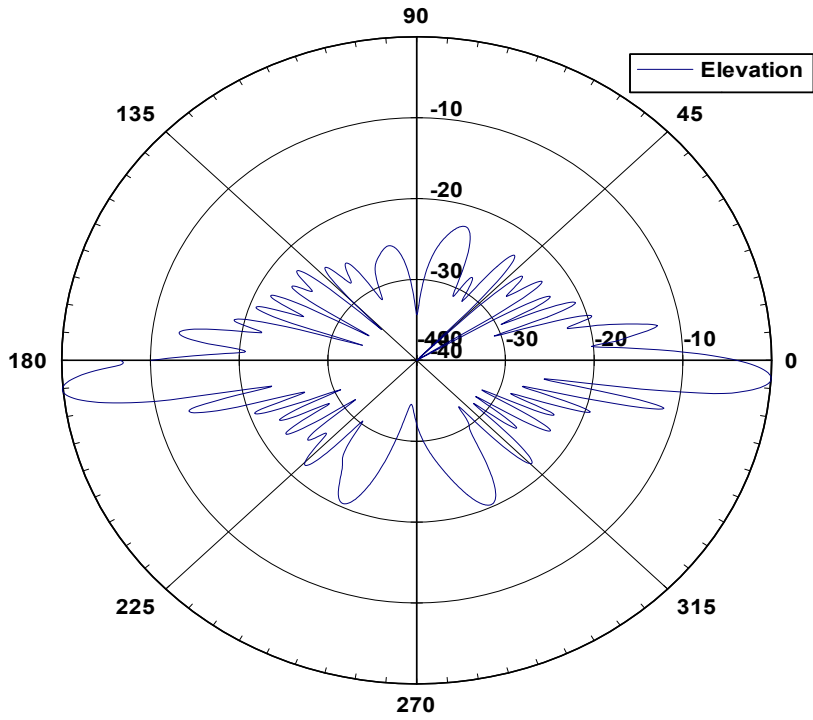
33 3360-2.5 Elevation Pattern
