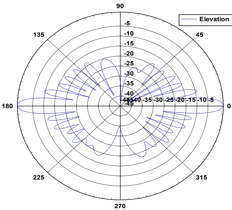
33 2360 Elevation Pattern
