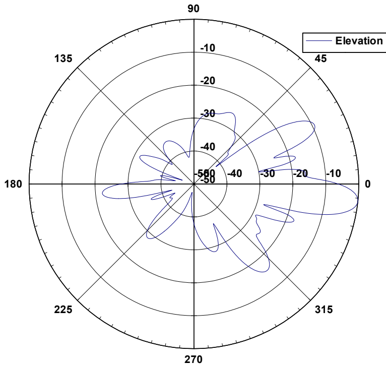
35 9008-6 XPXP-MIMO Elevation Pattern
