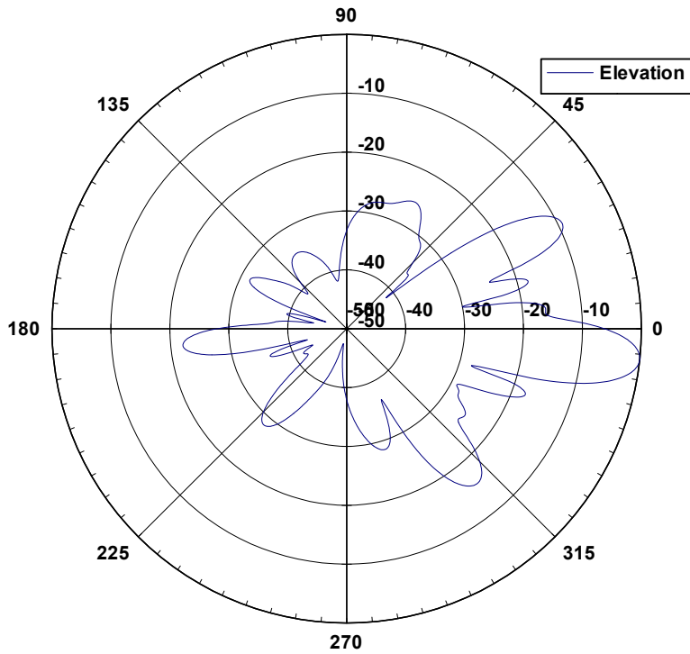
35 9008-6 XP Elevation Pattern
