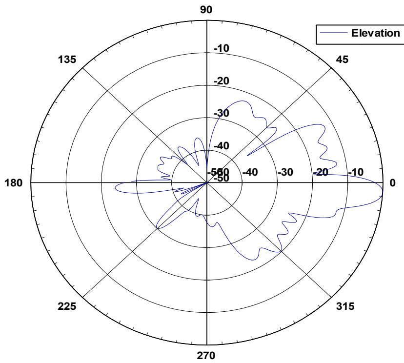
35 9008-4 XPXP-MIMO Elevation Pattern
