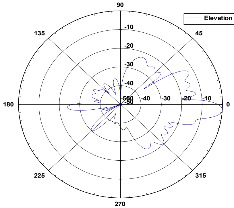
35 9008-4 XP Elevation Pattern
