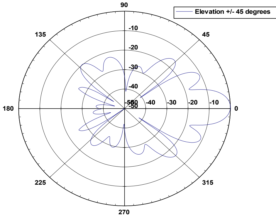
35 6015 XP Elevation Pattern
