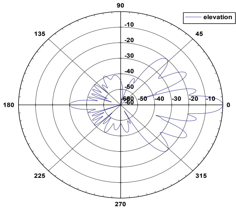
35 6008H Elevation Pattern
