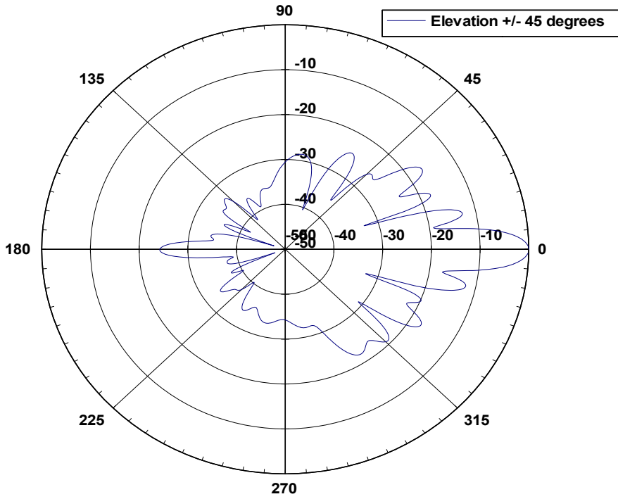
35 6008 XP Elevation Pattern
