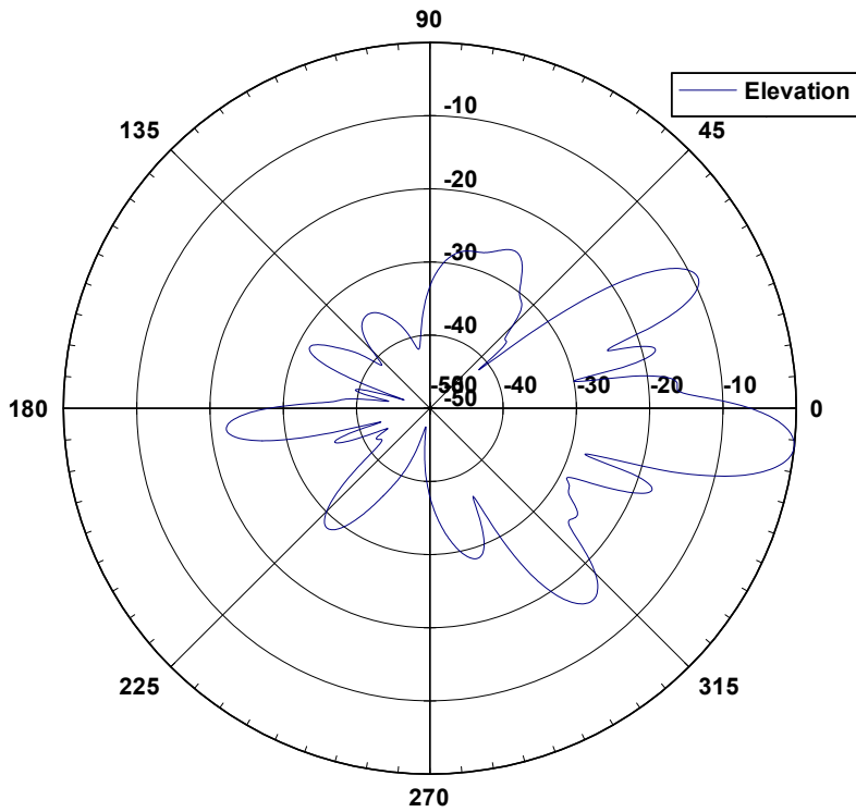
35 6008-6 XPXP-MIMO Elevation Pattern
