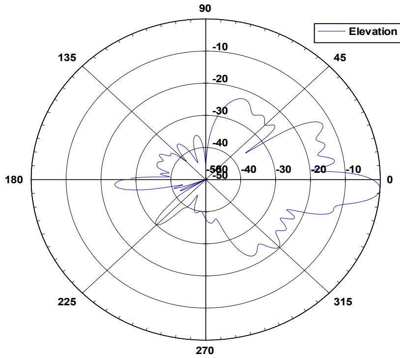
35 6008-4 XP Elevation Pattern
