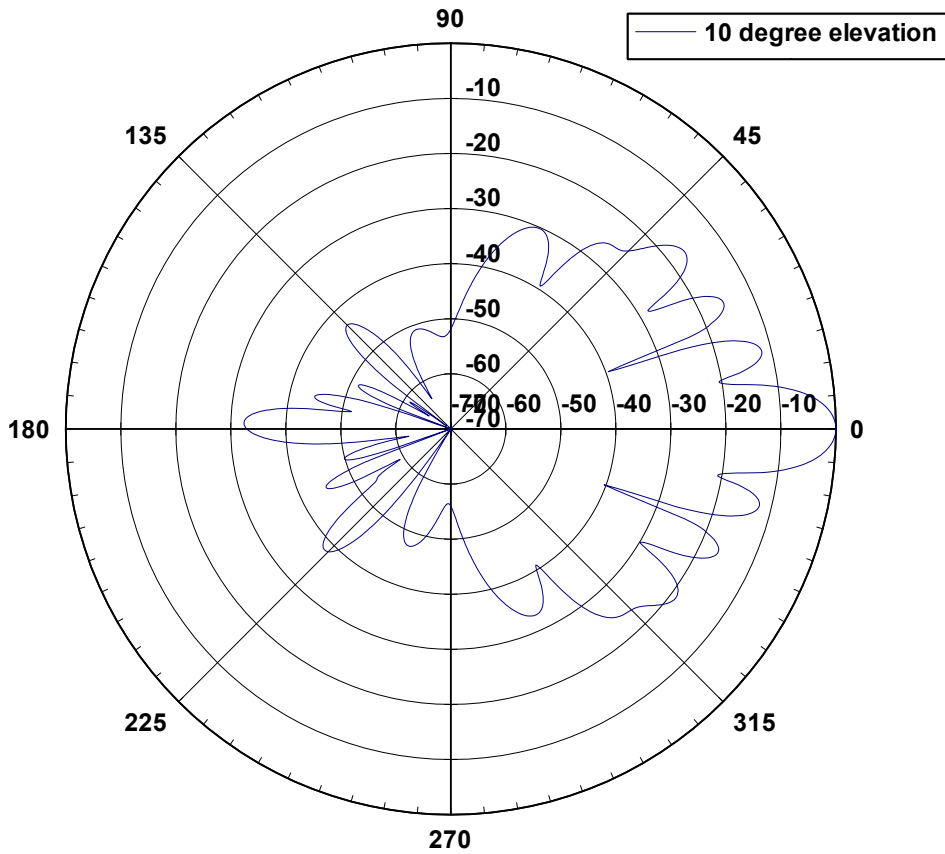
24 6010H Elevation Pattern
