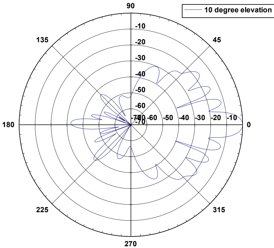
24 6010 Elevation Pattern
