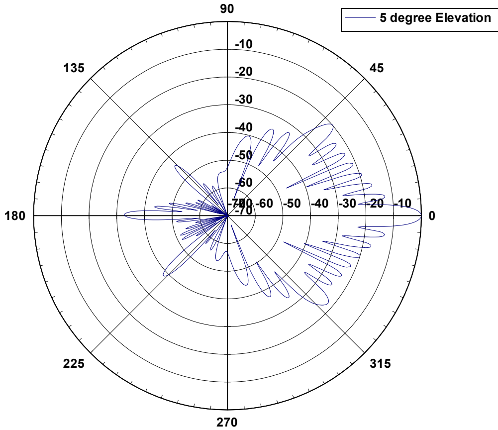
24 6005H Elevation Pattern
