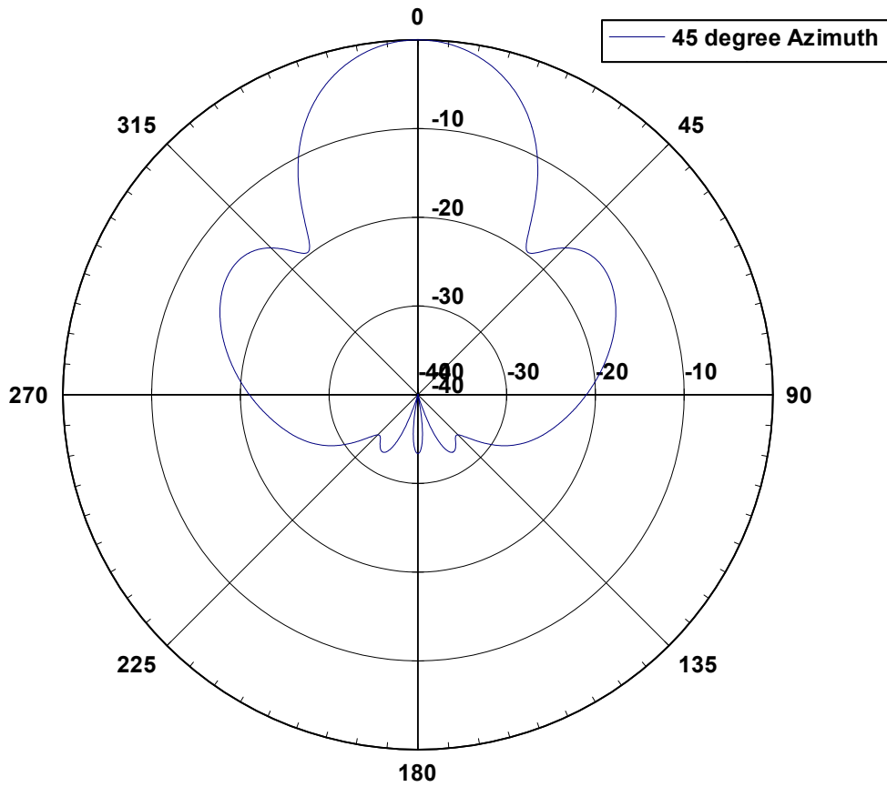
24 4510 Elevation Pattern
