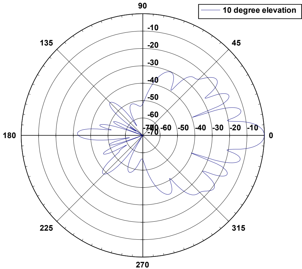
24 4510 Elevation Pattern
