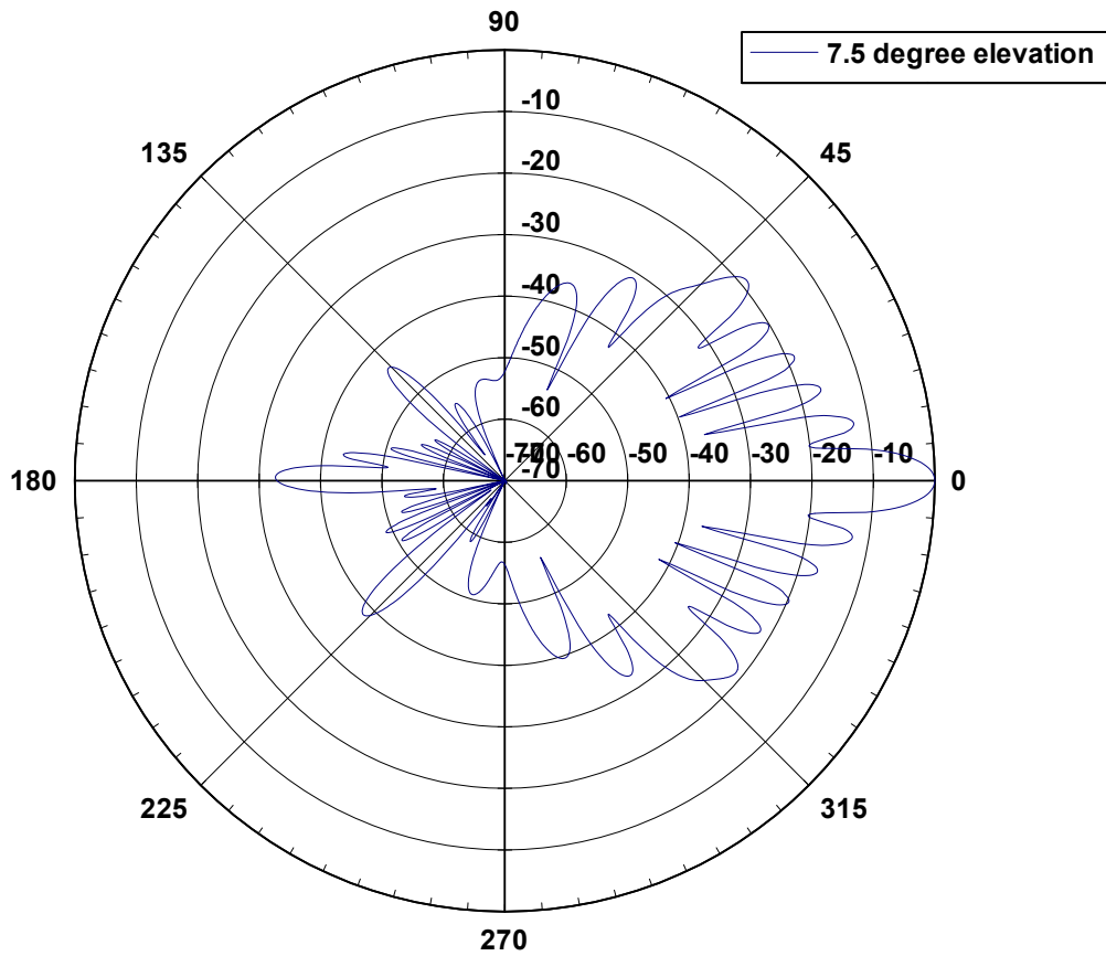
24 4507H Elevation Pattern
