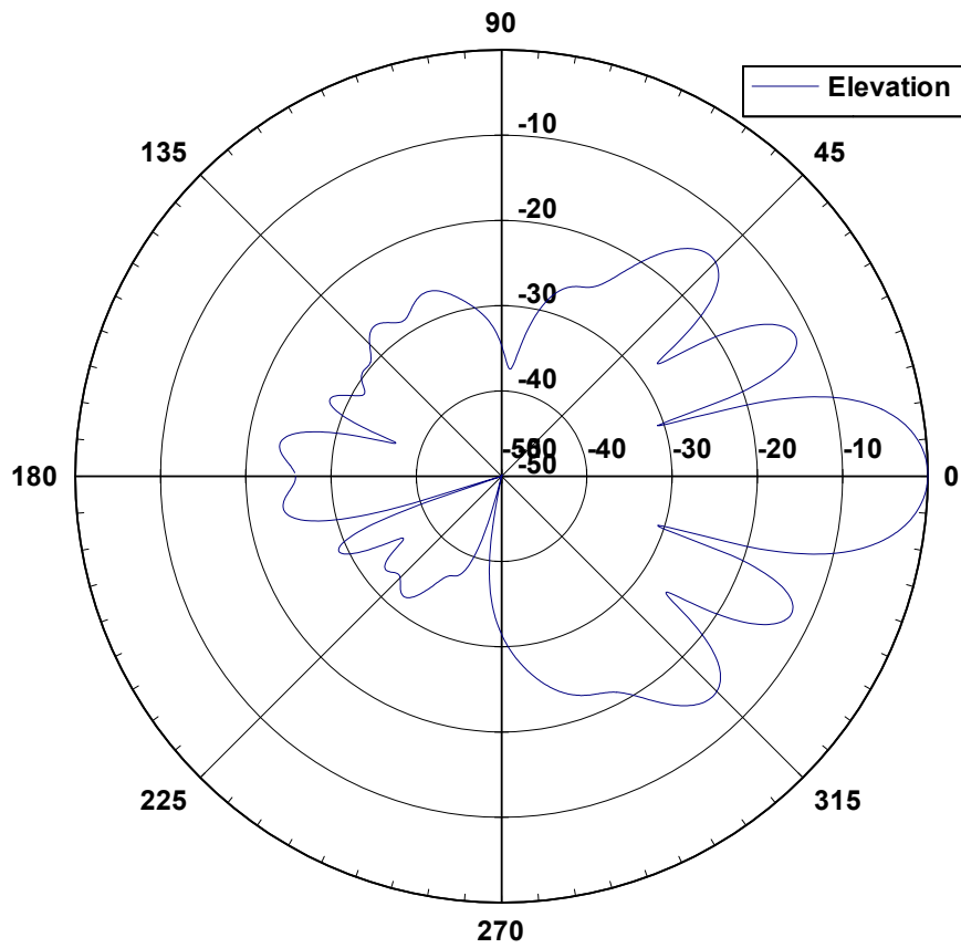
24 18015 Elevation Pattern
