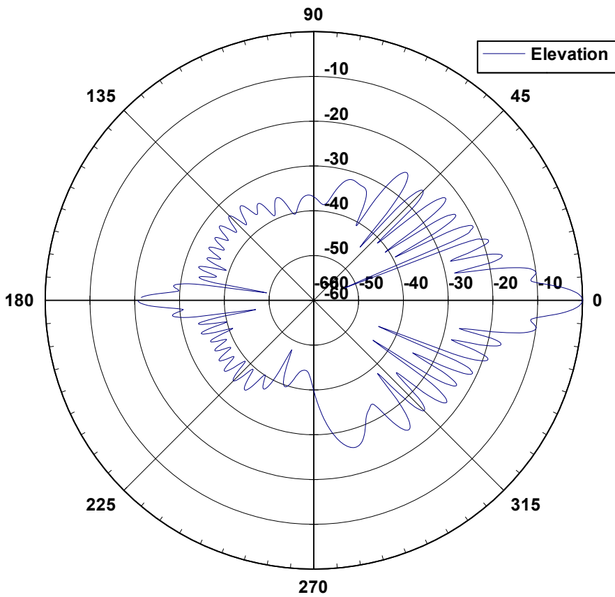
24 18005 Elevation Pattern
