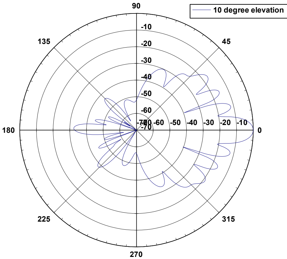
24 12010 Elevation Pattern
