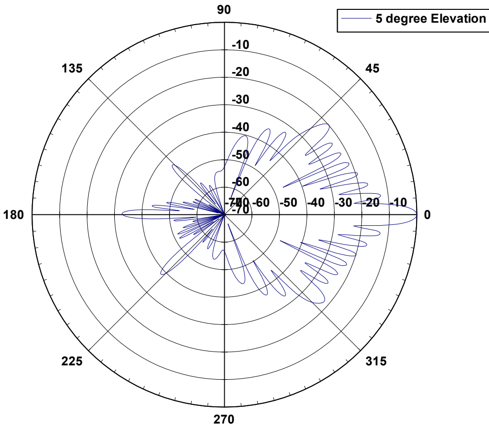
24 12005 Elevation Pattern
