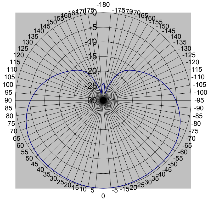
24 18015 10dbi Base Station Azimuth Pattern
