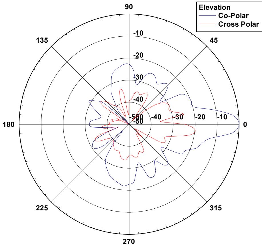
24 SD24 Elevation Pattern
