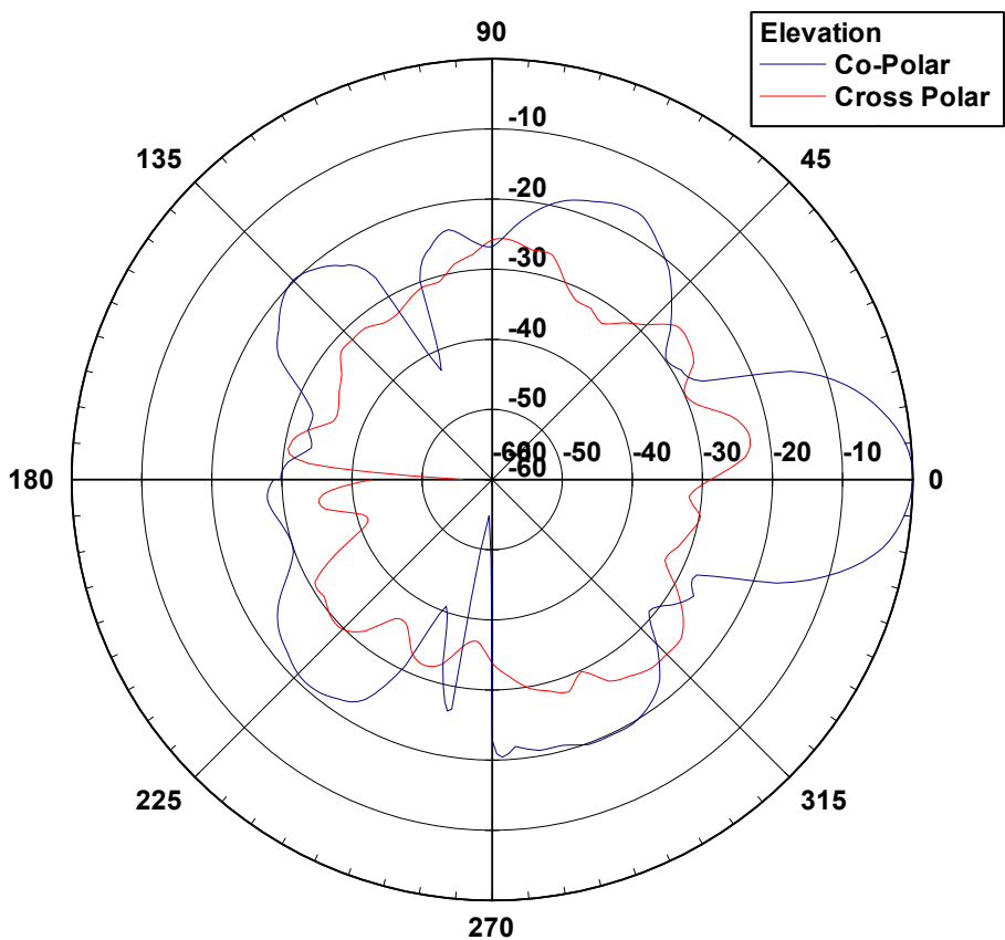
24 SD15 Elevation Pattern
