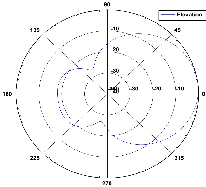
24 8080H OB Elevation Pattern
