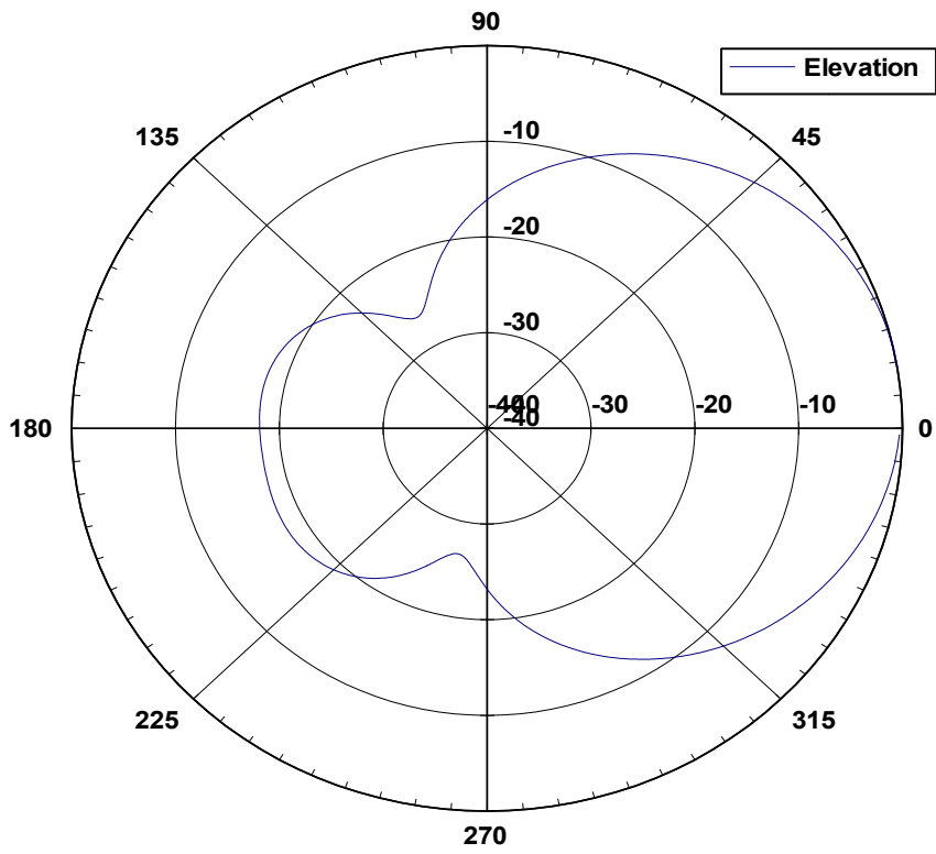
24 8080 OB Elevation Pattern
