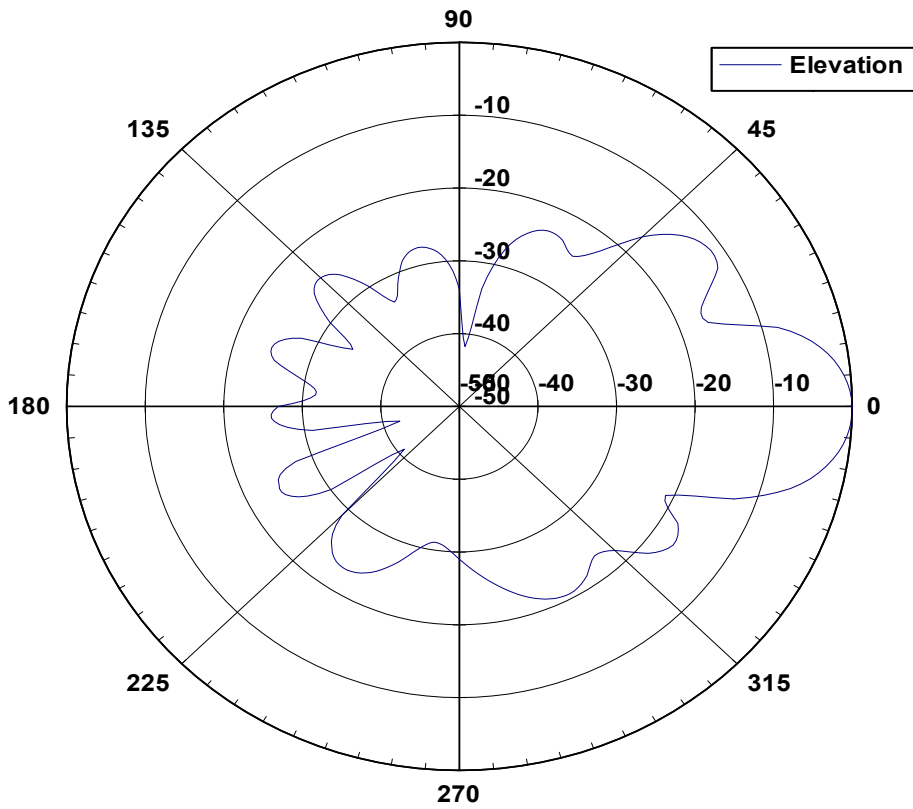
19 3030H Elevation Pattern
